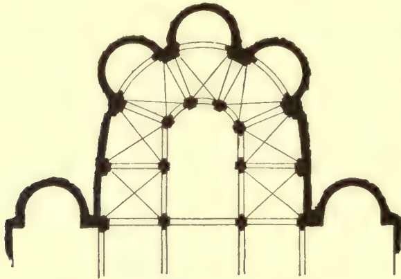
Fig. 327.—Aversa. Duomo. Plan of choir (about 1049–1078).
